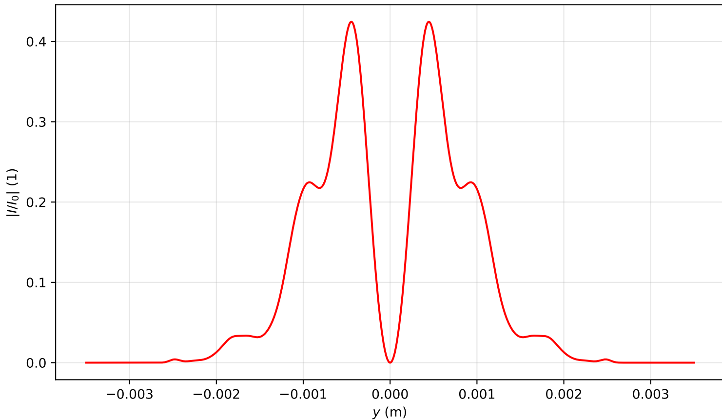
Intensity profile I(x=0, y, z=2.468)/I_0 , P_{in}=5.0P_{cr} , artificial time
